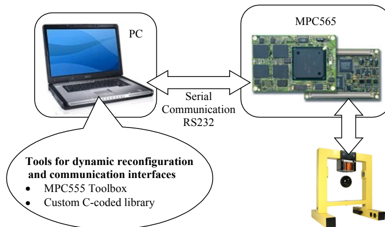
Fig. 5. Host – target control architecture and communication method.
