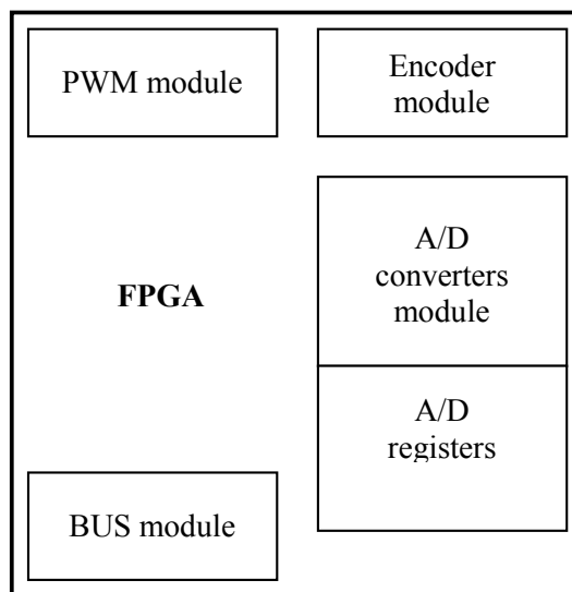
Fig. 3. User-defined FPGA core.
