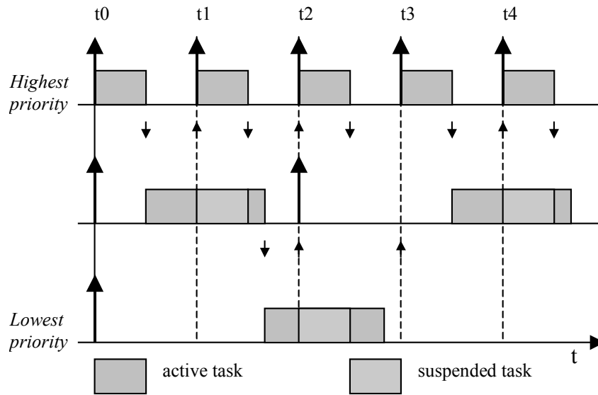
Fig. 2. Tasks execution in the multitasking mode.
