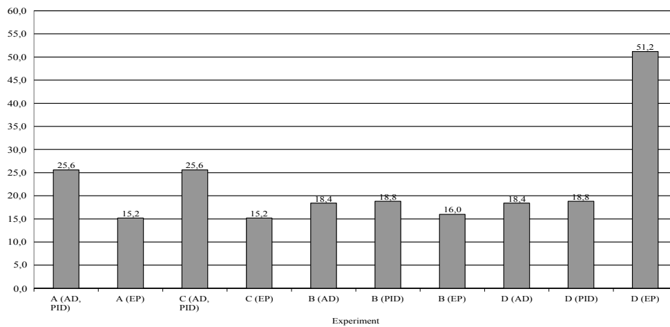
Fig. 8. Maximum turnaround time [μs].
