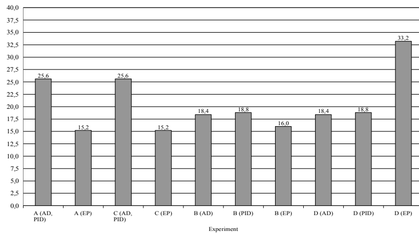
Fig. 9. Maximum execution time [μs].
