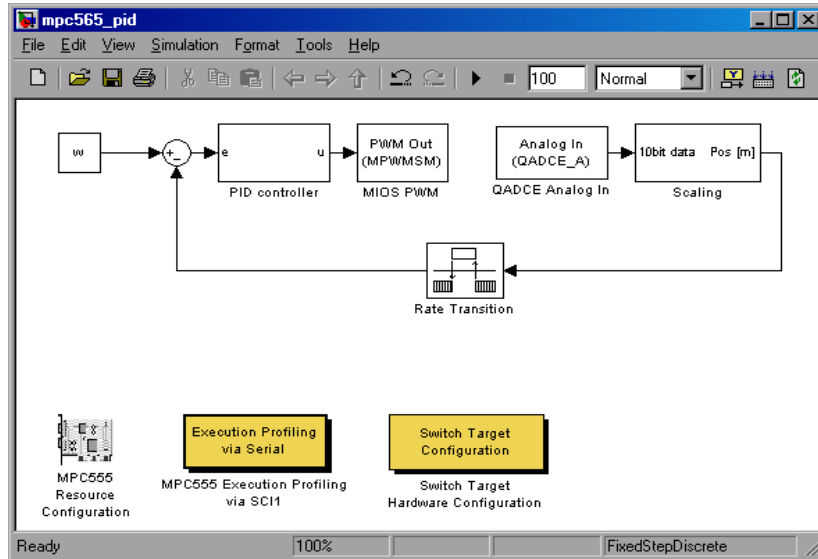
Fig. 6. PID Control loop algorithm designed in Simulink and prepared for MPC565 code generation.
